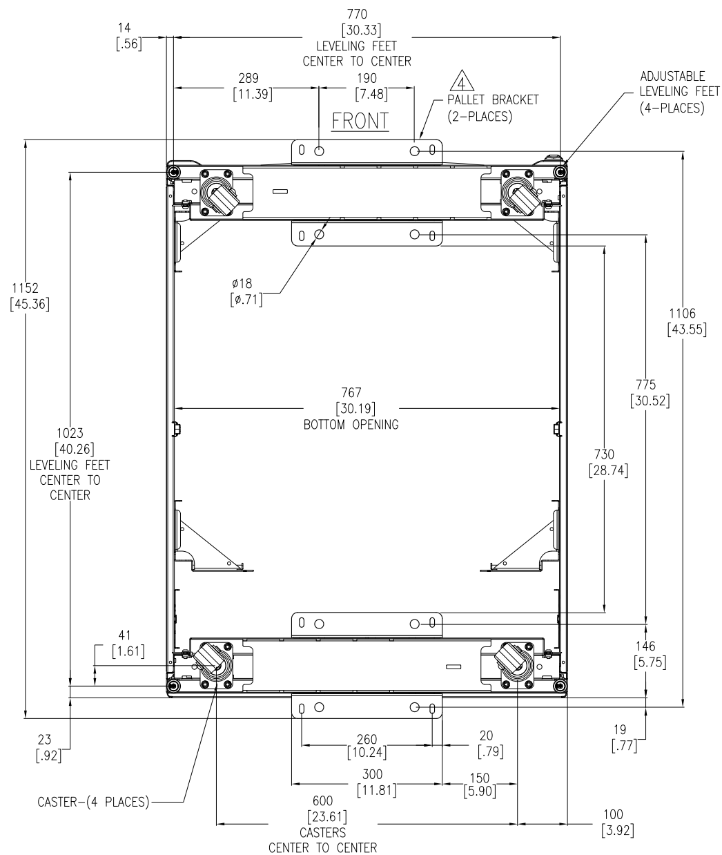
BOTTOM VIEW (WITH PALLET BRACKETS, CAN BE USED FOR ANCHORING) TOP ROOF NOT SHOWN
